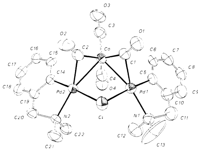
Figure 2. The molecular geometry of [\text{Pd}(\text{NMe}_2\text{CH}_2\text{C}_6\text{H}_4)_2\mu\{\text{Co}(\text{CO})_4\mu\text{Cl}] , including the atomic-numbering scheme. Bond lengths: Pd1–Co 2.597 (1), Pd2–Co 2.595 (1), Pd1–Cl 2.434 (2), Pd2–Cl 2.434 (2), Pd1–Cl 2.170 (8), Pd2–C2 2.138 (9), Co–C1 1.780 (8), and Co–C2 1.809 (8) Å. Angles: Pd1–Co–Pd2 83.1 (6), Pd2–Cl–Pd2 90.01 (7), Co–C1–O1 156.6 (8), and Co–C2–O2 154.8 (7)°.
